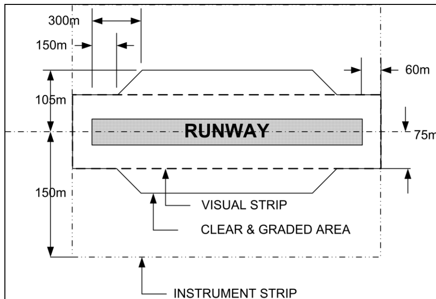
Figure 5-1 Graded portion of a runway strip
