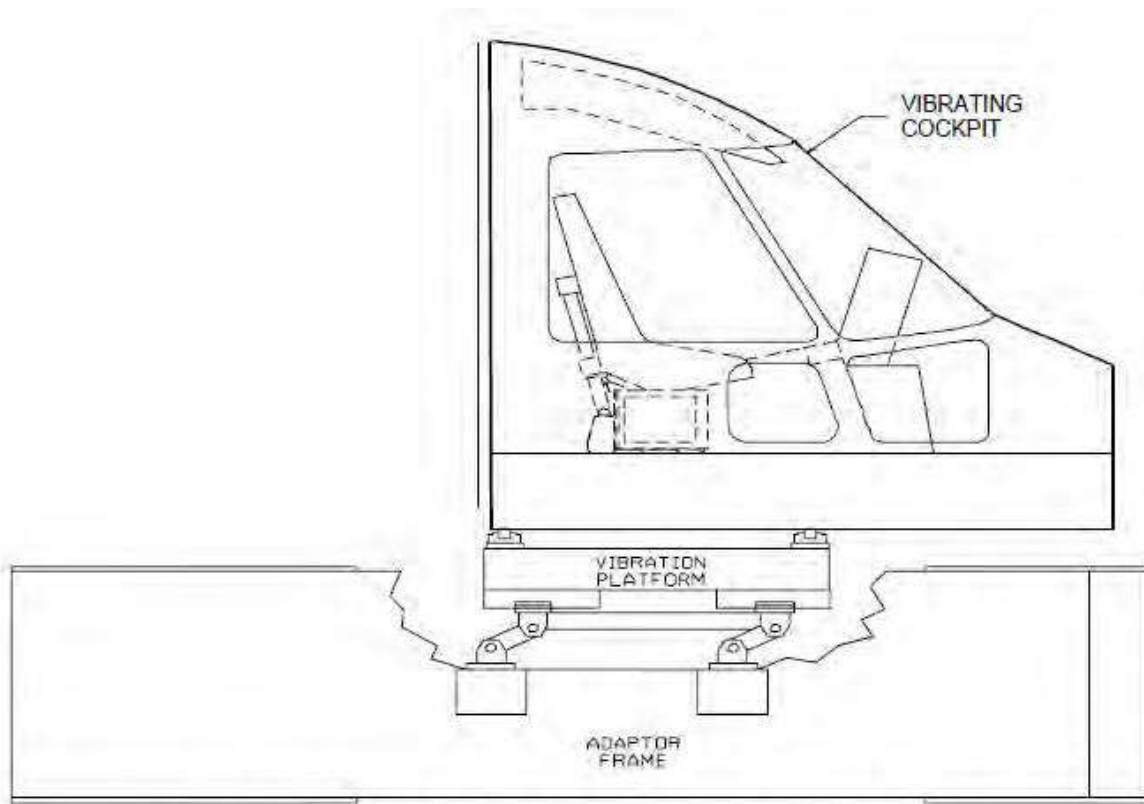
Figure 1: An Example of a three degree of freedom cockpit vibration system
