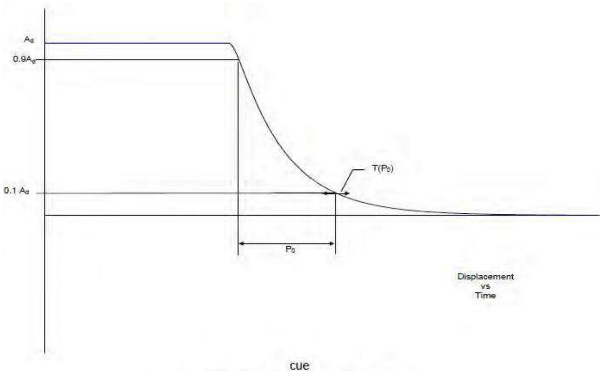
Figure 2: Critically damped step response
