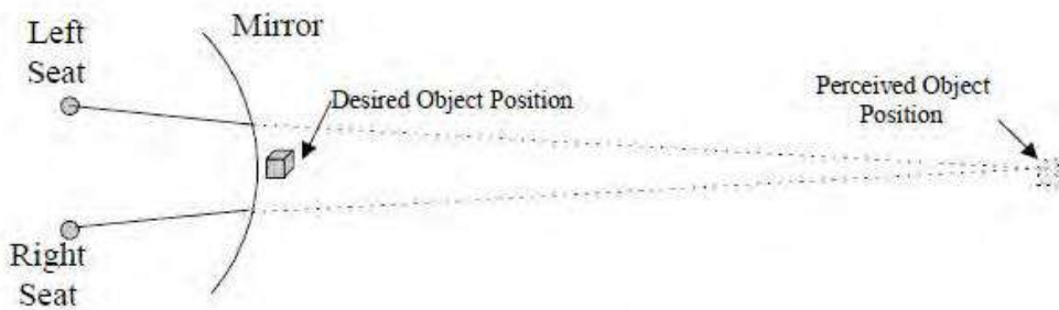
Figure 4 - Near field object in a collimated display
