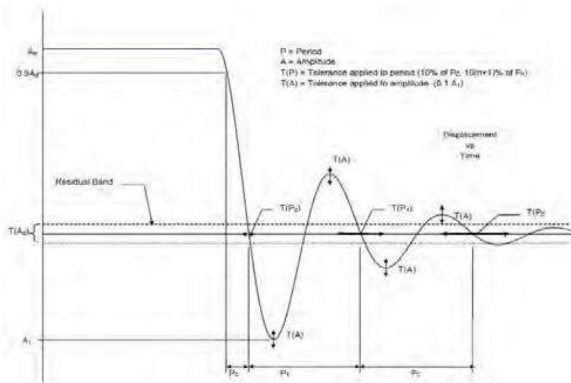
Figure 1: Underdamped step response
